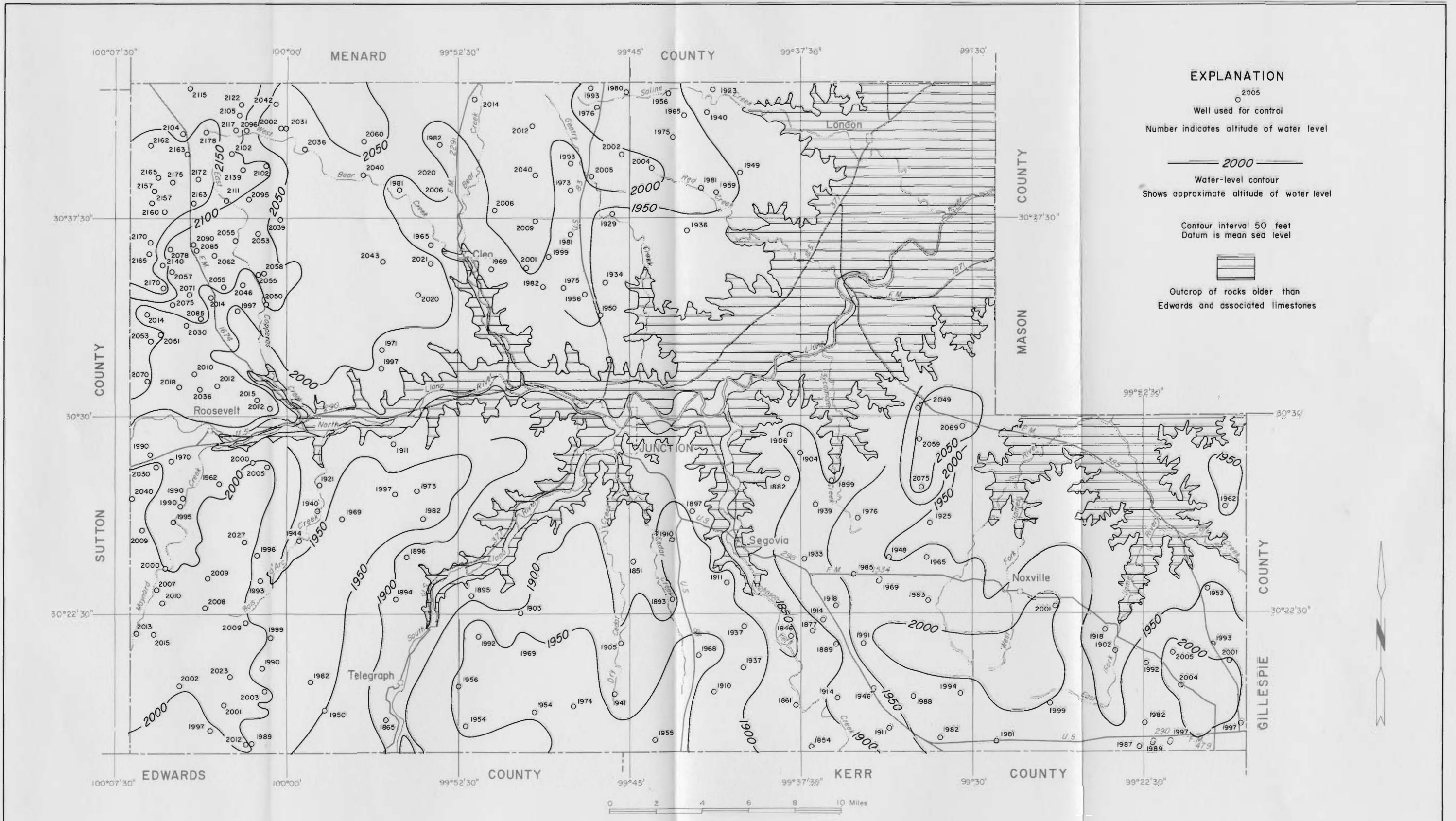
Figure 8 Approximate Altitude of Water Levels in the Edwards and Associated Limestones in 1966
